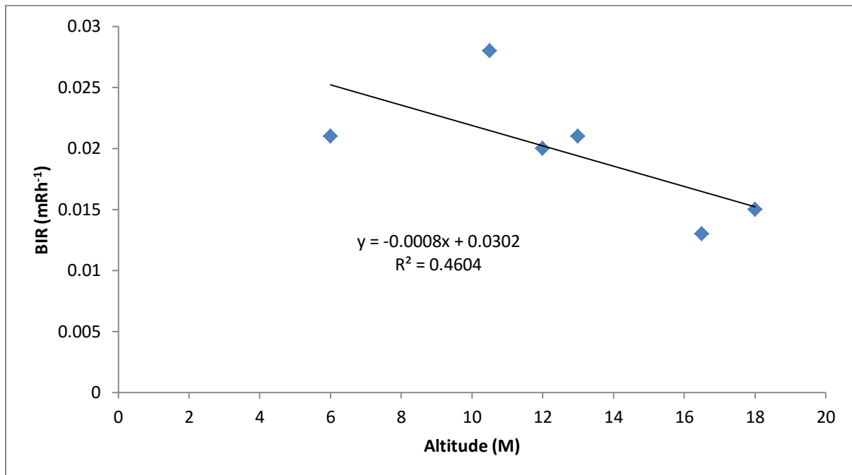
Fig. 5: Correlation between Exposure rate and the Elevation
