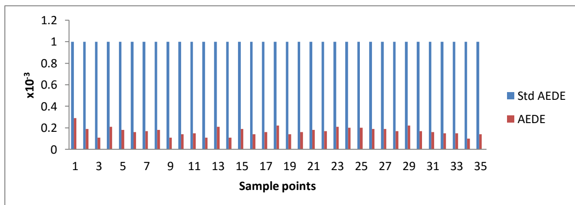
Fig. 3: Comparison of standard AEDE and measured AEDE
