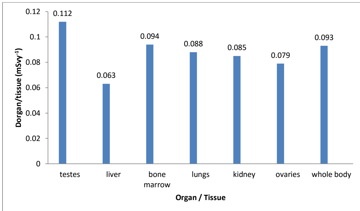
Fig. 4: Chart of Effective dose to Human Organ or Tissue
